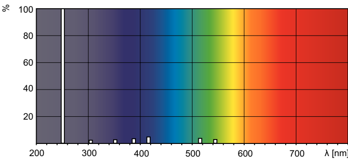
Spectral Power Distribution Colour - TUV 335W WP XPT SE UNP
