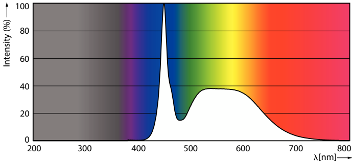
Spectral Power Distribution Colour - MAS LEDtube 1500mm HO 16.7W 865 T8 EELB
