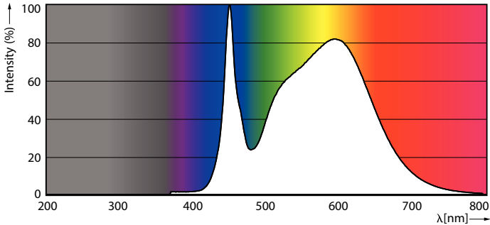
Spectral Power Distribution Colour - MAS LEDtube HF 1500mm UO 24W840 T8
