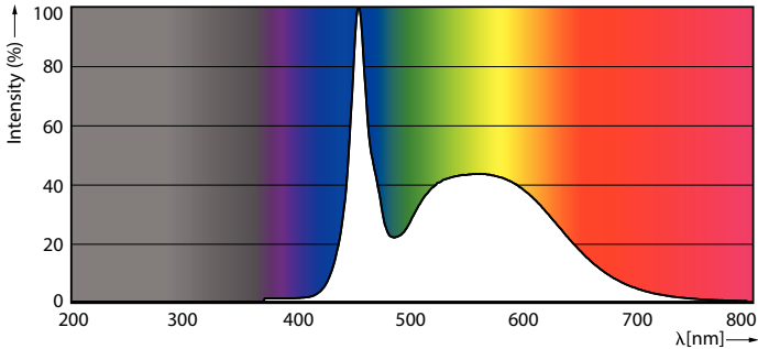
Spectral Power Distribution Colour - MAS LEDtube HF 1200mm UO 16W865 T8
