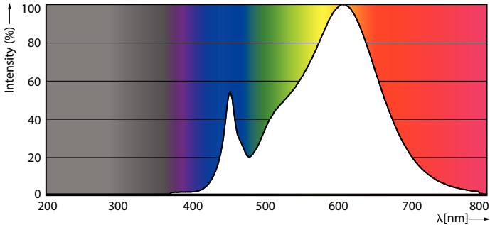
Spectral Power Distribution Colour - MAS LEDtube HF 1500mm HO 26W 830 T5 OE
