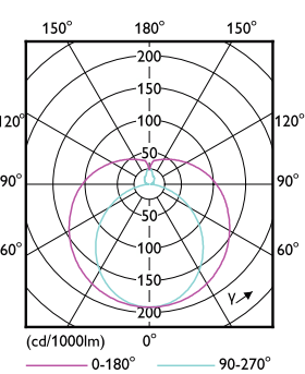
Light Distribution Diagram - MAS LEDtube VLE 600mm HO 8W 865 T8
