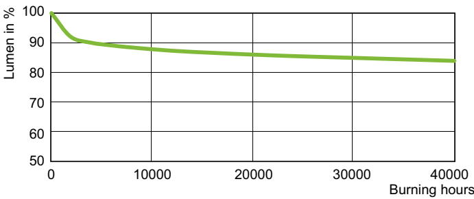
Lumen Maintenance Diagram - MST SON-T APIA Plus Xtra 70W E27 1SL/12
