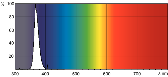
Spectral Power Distribution Colour - TL-D 18W BLB 1SL/25
