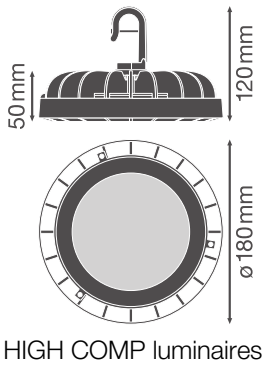
HIGH COMP luminaires
